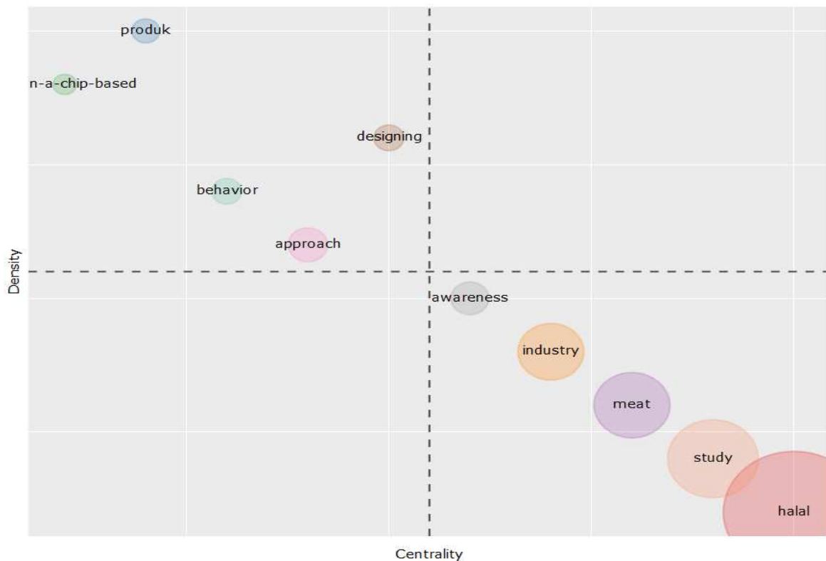
Figure 14: Thematic Map
