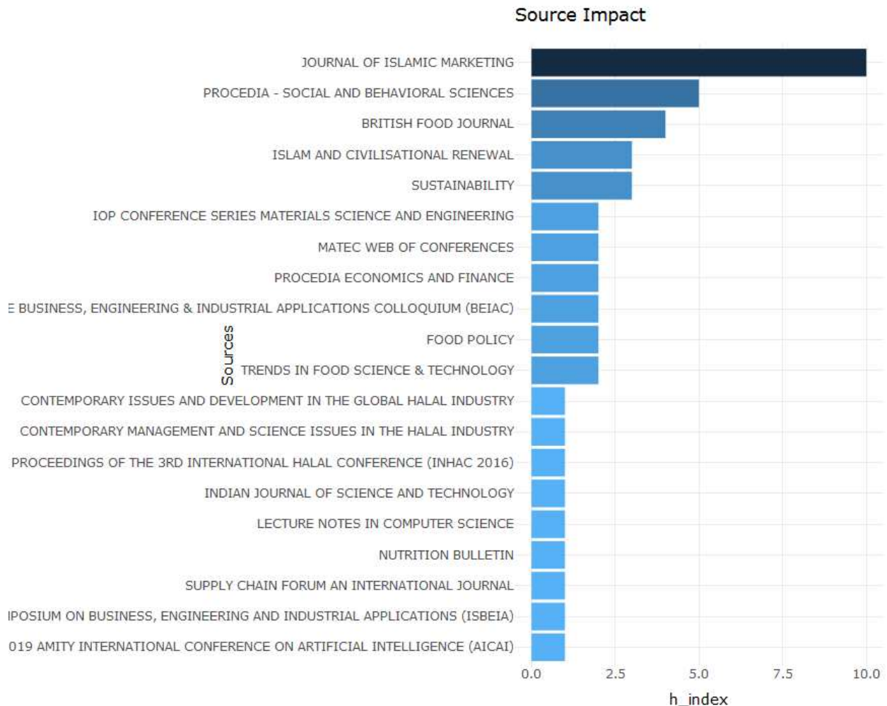
Figure 3: Source Impact
