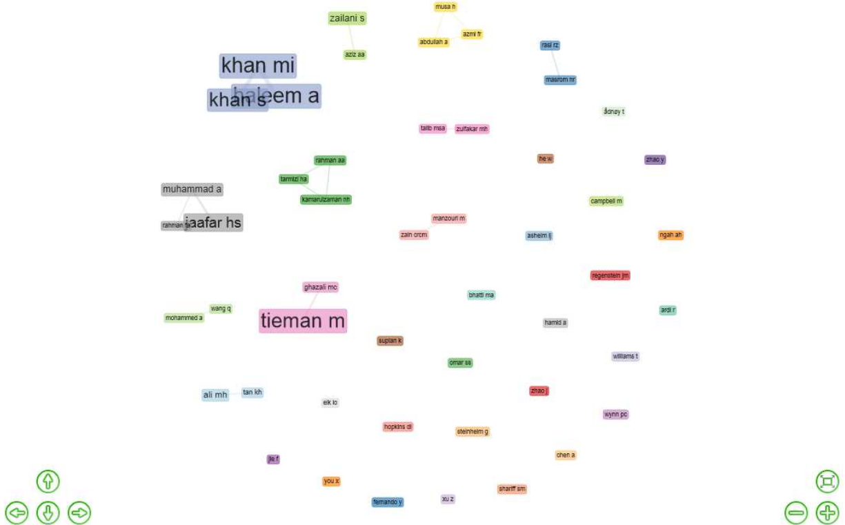
Figure 18: Collaboration Network
