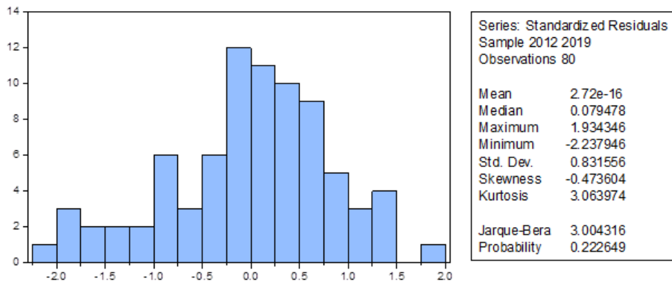
Figure 3.1. Normality Test
