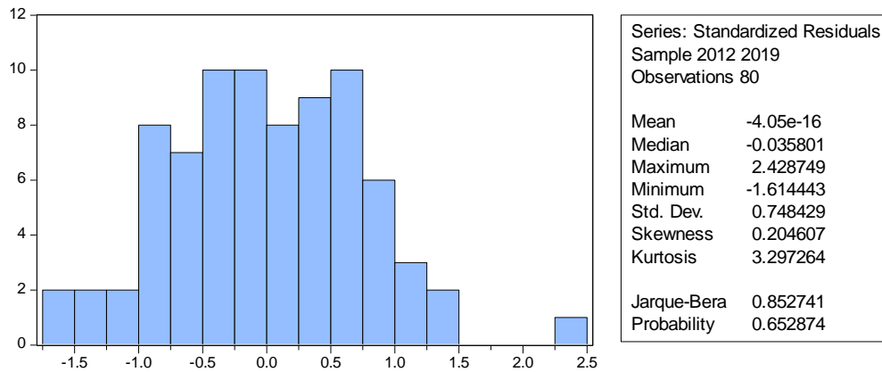
Figure 3.2 Normality Test
